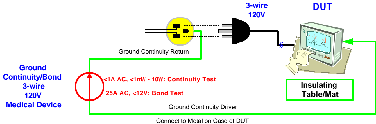
Figure 1.0a: Ground Continuity/Bond Test
